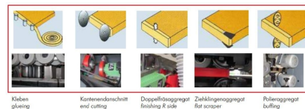
Kleben gluing
